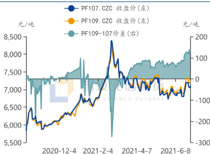
图6: PF109-107价差
